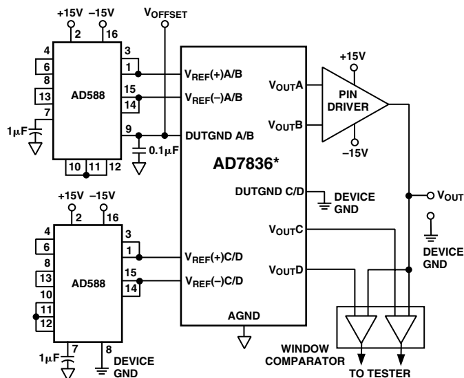
Figure 21. ATE Application
