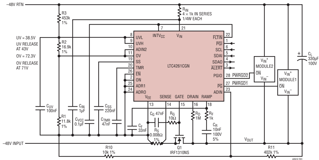
Figure 1. -48\text{V}/200\text{W} Hot Swap Controller Using LTC4261 with Current, Input Voltage and V_{DS} Monitoring (5.6A Current Limit, 0.66A Inrush)
