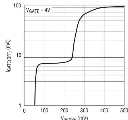
GATE Turn-Off Current vs SENSE Voltage
