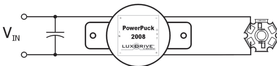
Figure 17. Place a capacitor across the input terminals when the distance to the DC power source is greater than 18 inches
