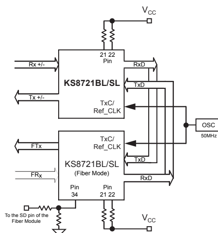
Figure 3. Fiber Module
