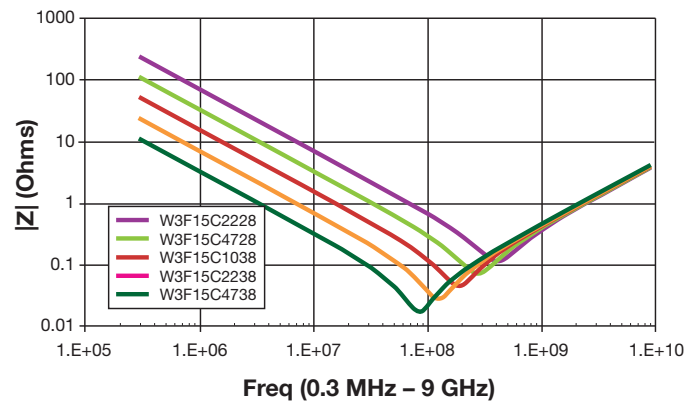
IMPEDANCE 1206 – 50V
