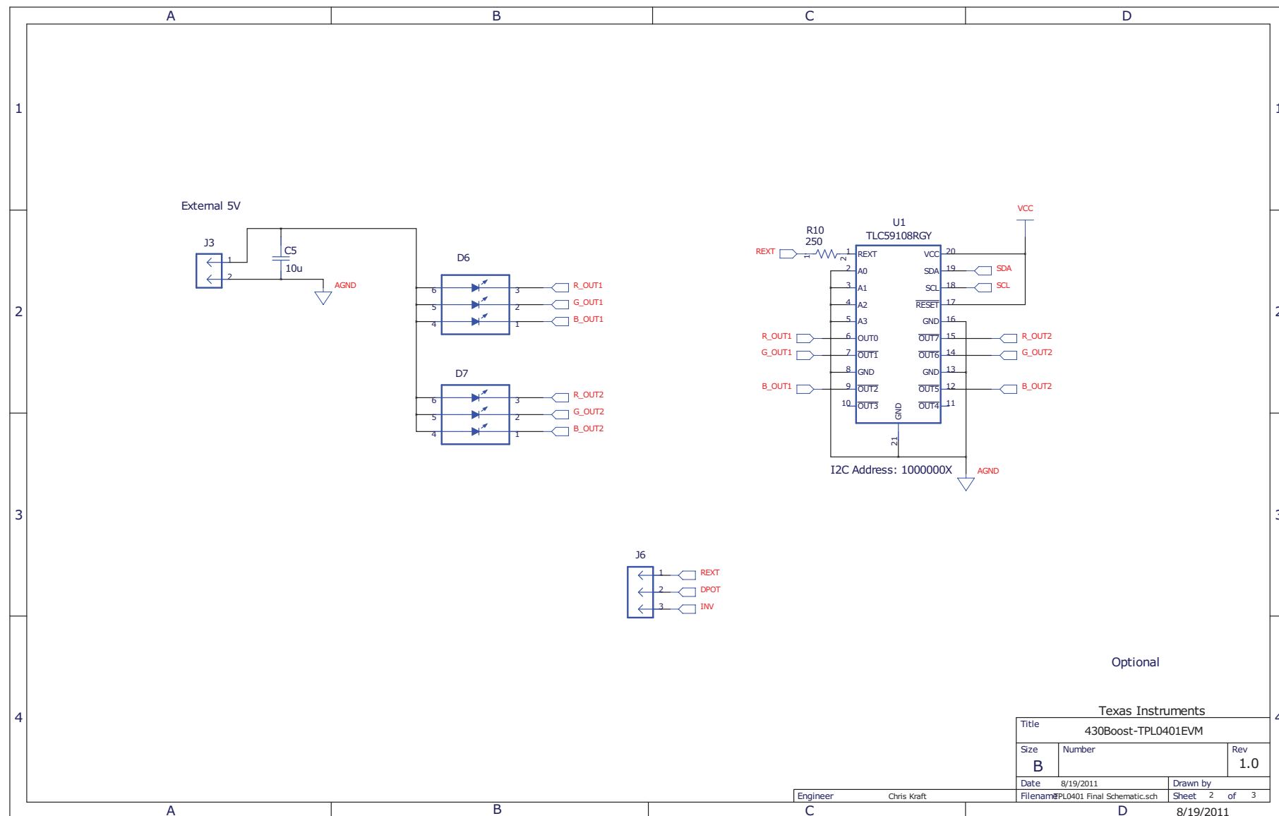
Figure 4. TLC59108 Schematic
