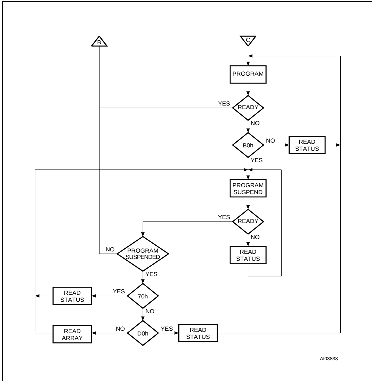
Figure 31. Command Interface and Program Erase Controller Flowchart (d)
