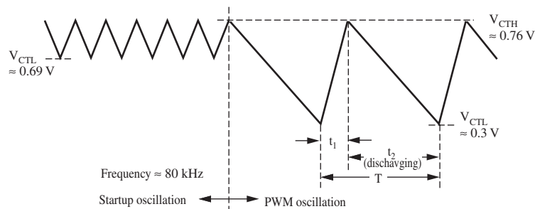
Figure 1-1. Triangular oscillation waveform
