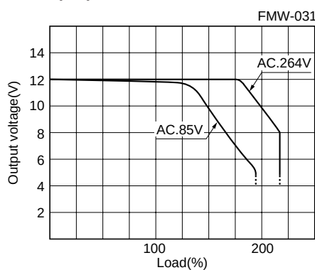
+12V output(25°C, 5V • 3.4A, -12V • 0.3A OUTPUT)
