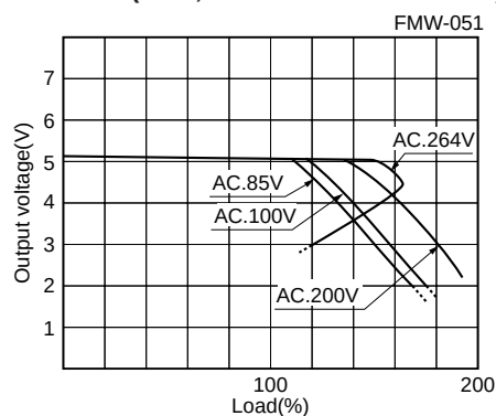
+5V OUTPUT(25°C, ±12V OUTPUT RATINGS)
