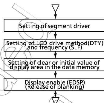
Figure 3-36. Initial setting of LCD driver
