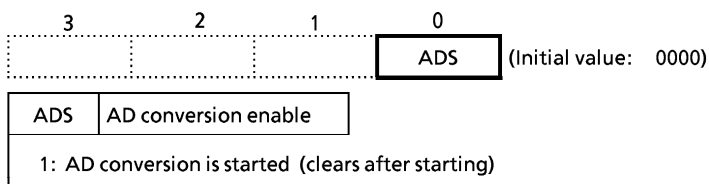
Figure 3-22. AD conversion start register
