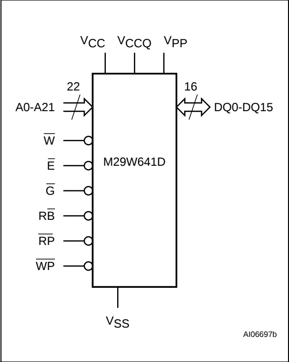
Figure 2. Logic Diagram
