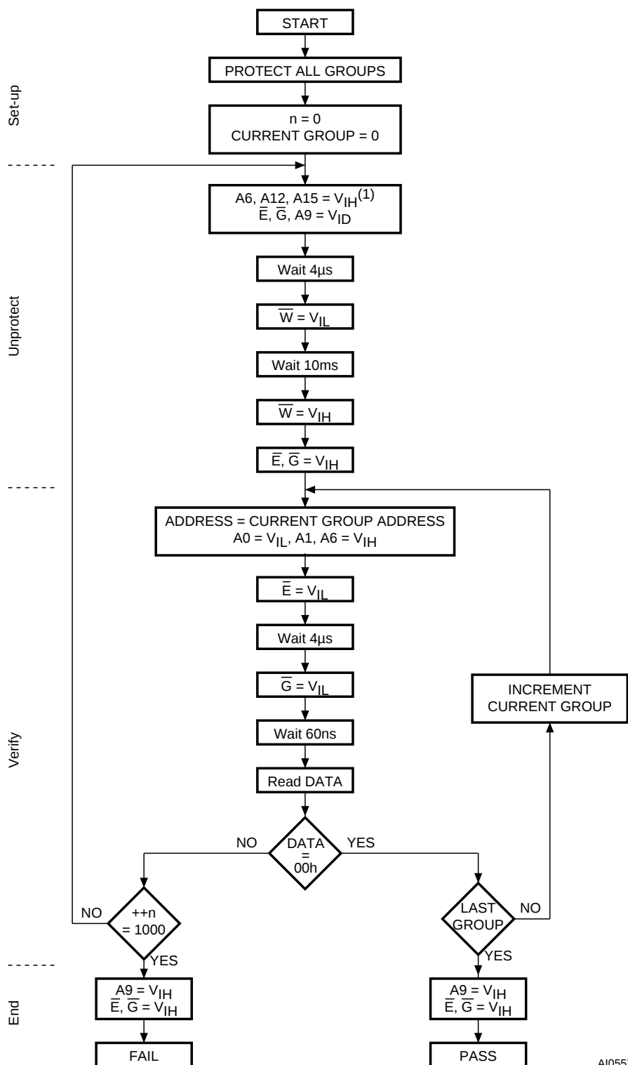
Figure 17. Programmer Equipment Chip Unprotect Flowchart
