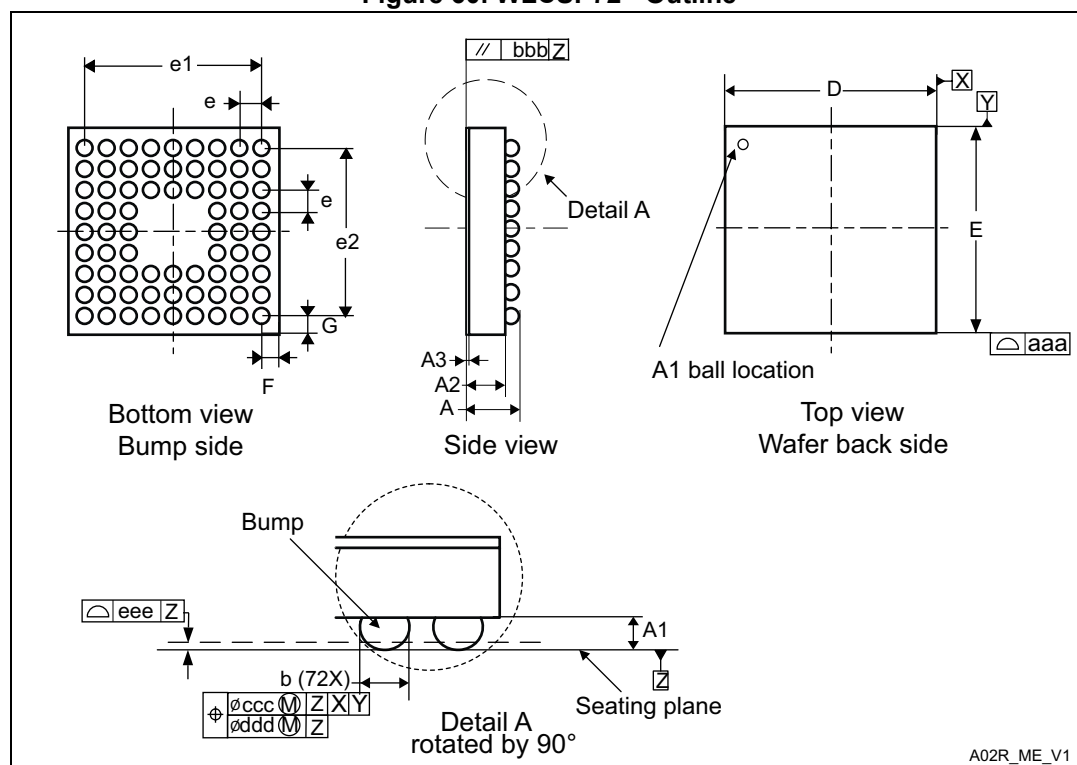
Figure 60. WLCSP72 - Outline
