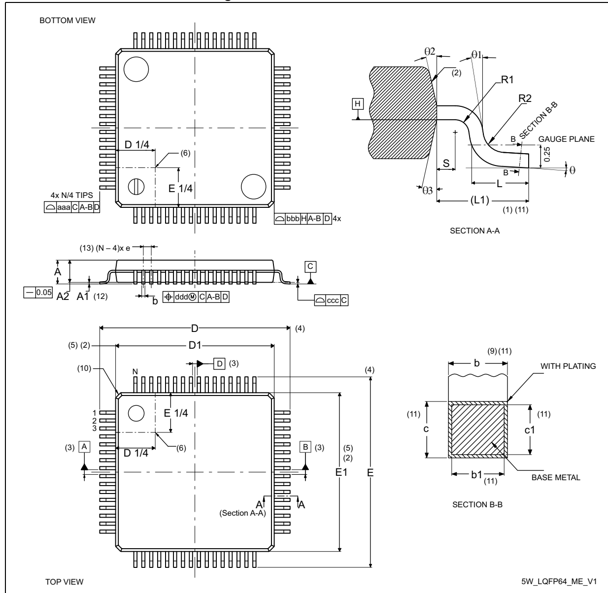
Figure 63. LQFP64 - Outline (15)
