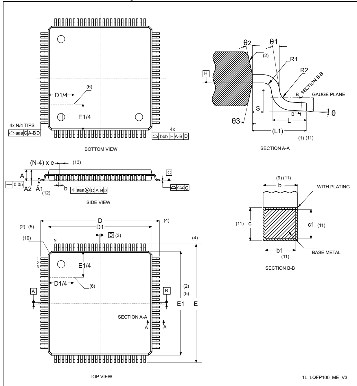
Figure 58. LQFP100 - Outline (15)
