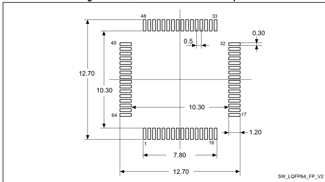
Figure 64. LQFP64 - Recommended footprint
