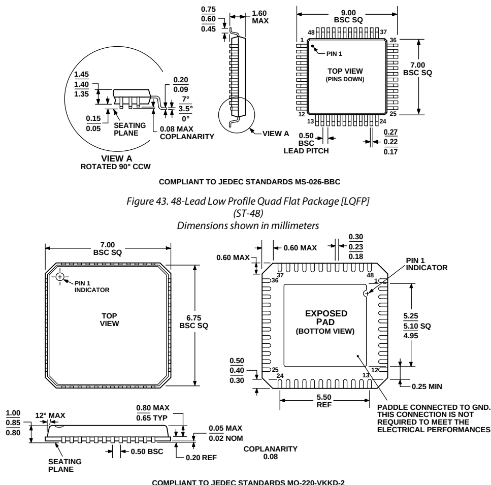
Figure 44. 48-Lead Lead Frame Chip Scale Package [LFCSP_VQ] 7 mm × 7 mm Body, Very Thin Quad (CP-48-1)
