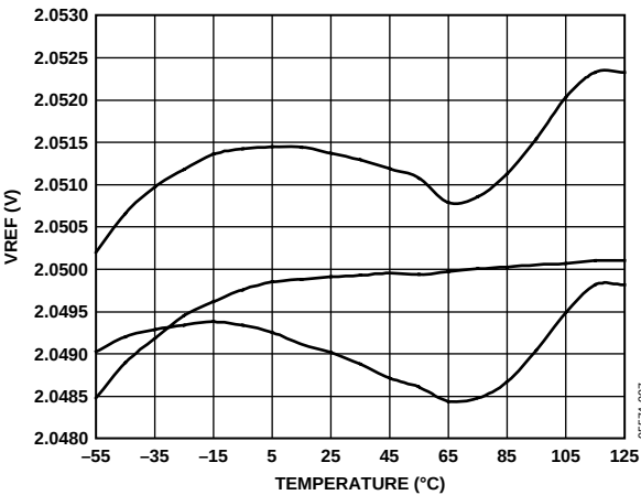
Figure 7. Typical Reference Voltage Output vs. Temperature (3 Units)
