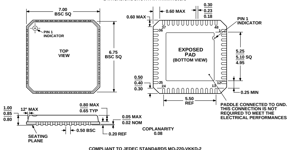
Figure 44. 48-Lead Lead Frame Chip Scale Package [LFCSP_VQ] 7 mm × 7 mm Body, Very Thin Quad (CP-48-1)
