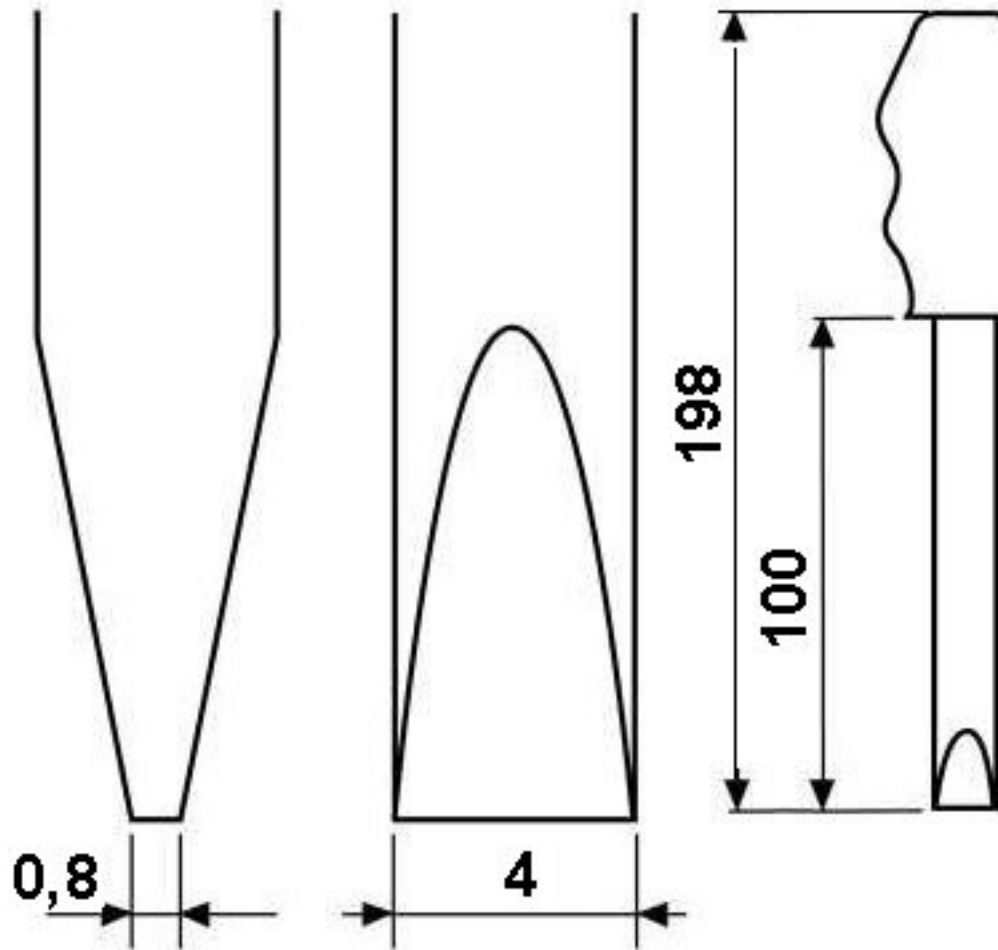
Dimensioned drawing
