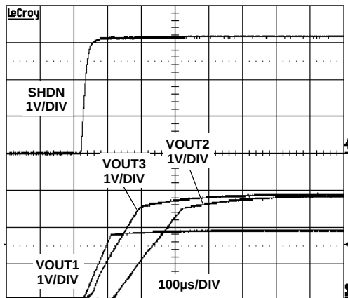
FIGURE 1. START-UP SEQUENCE
