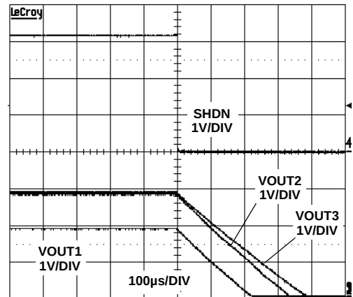
FIGURE 2. SHUTDOWN SEQUENCE
