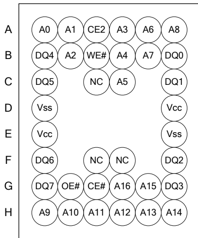
TFBGA(See through with Top View)
