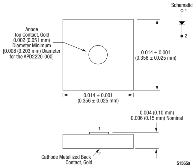
Figure 9. 149-815 Package
