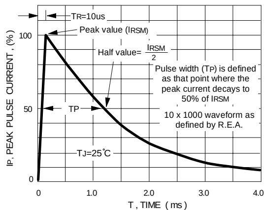
FIG.5 - PULSE WAVEFORM
