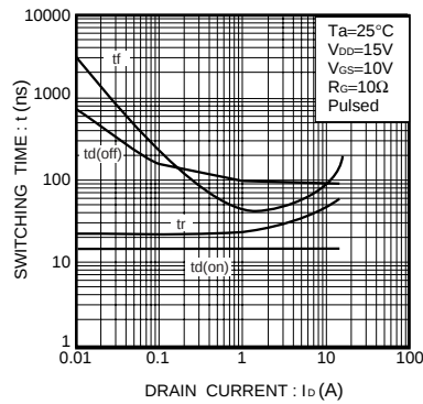
Fig.2 Switching Characteristics
