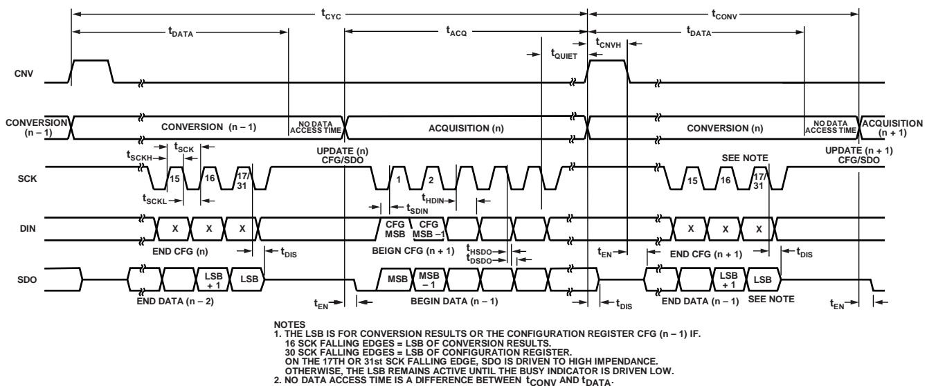
Figure 42. Serial Interface Timing for the AD7699 with a Busy Indicator
