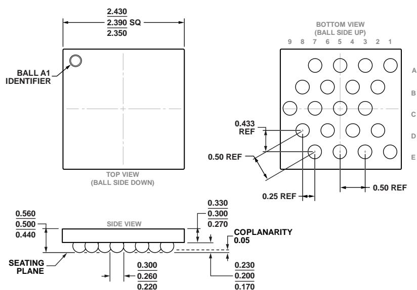
Figure 45. 20-Ball Wafer Level Chip Scale Package (WLCSF) (CB-20-12) Dimensions shown in millimeters
