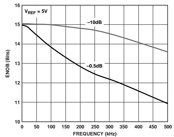
Figure 16. ENOB vs. Frequency
