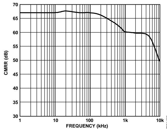
Figure 32. Analog Input CMRR vs. Frequency
