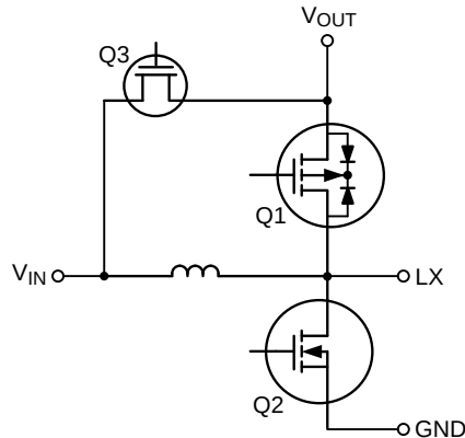
Figure 2. Boost Converter With Bypass Mode
