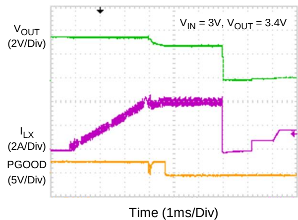
Overload Protection
