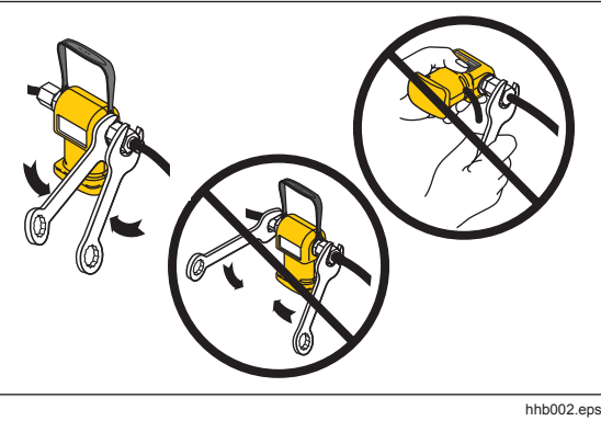
Figure 2. Applying Torque
