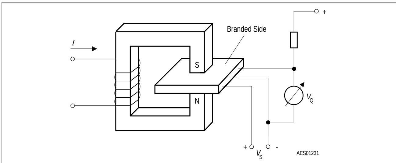
Figure 5 Sensor/Magnetic-Field Configuration
