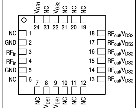
Figure 2. Pin Connections
