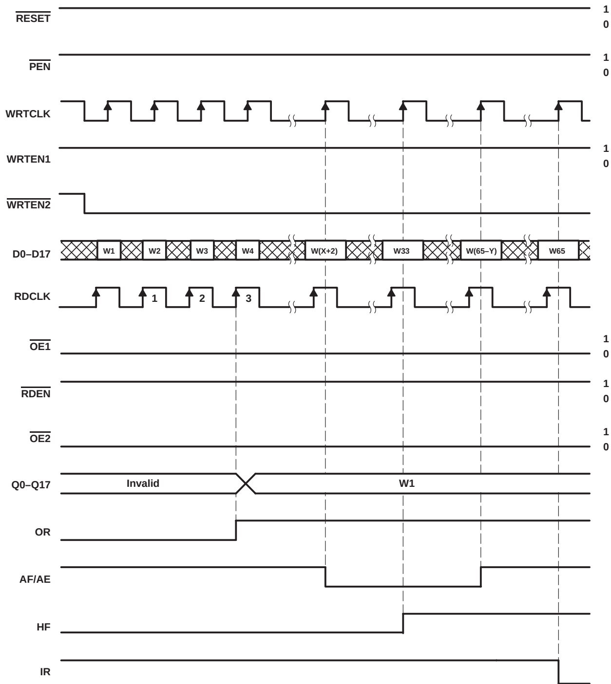
Figure 2. Write Cycle
