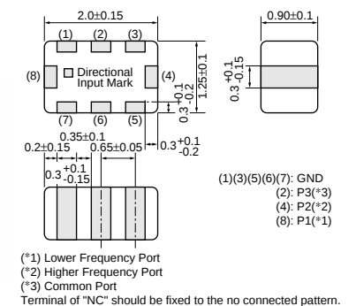
LFD21 DP4 Series
