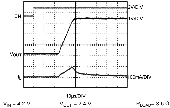
Figure 30. Start-Up
