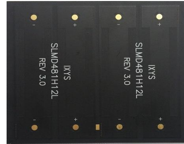
Back-side View
