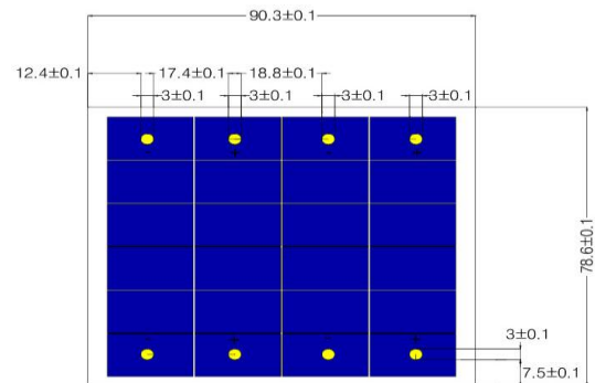
Back-side View
