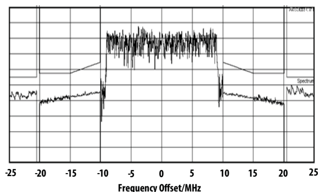
Figure 24. SEM at Pout=29dBm @ 1.87GHz
