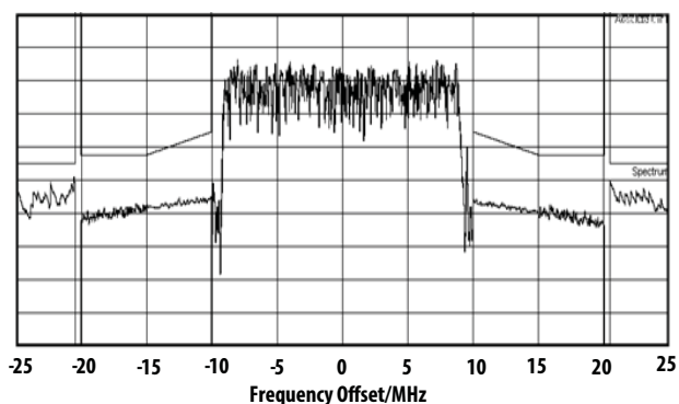
Figure 23. SEM at Pout=29dBm @ 1.842GHz
