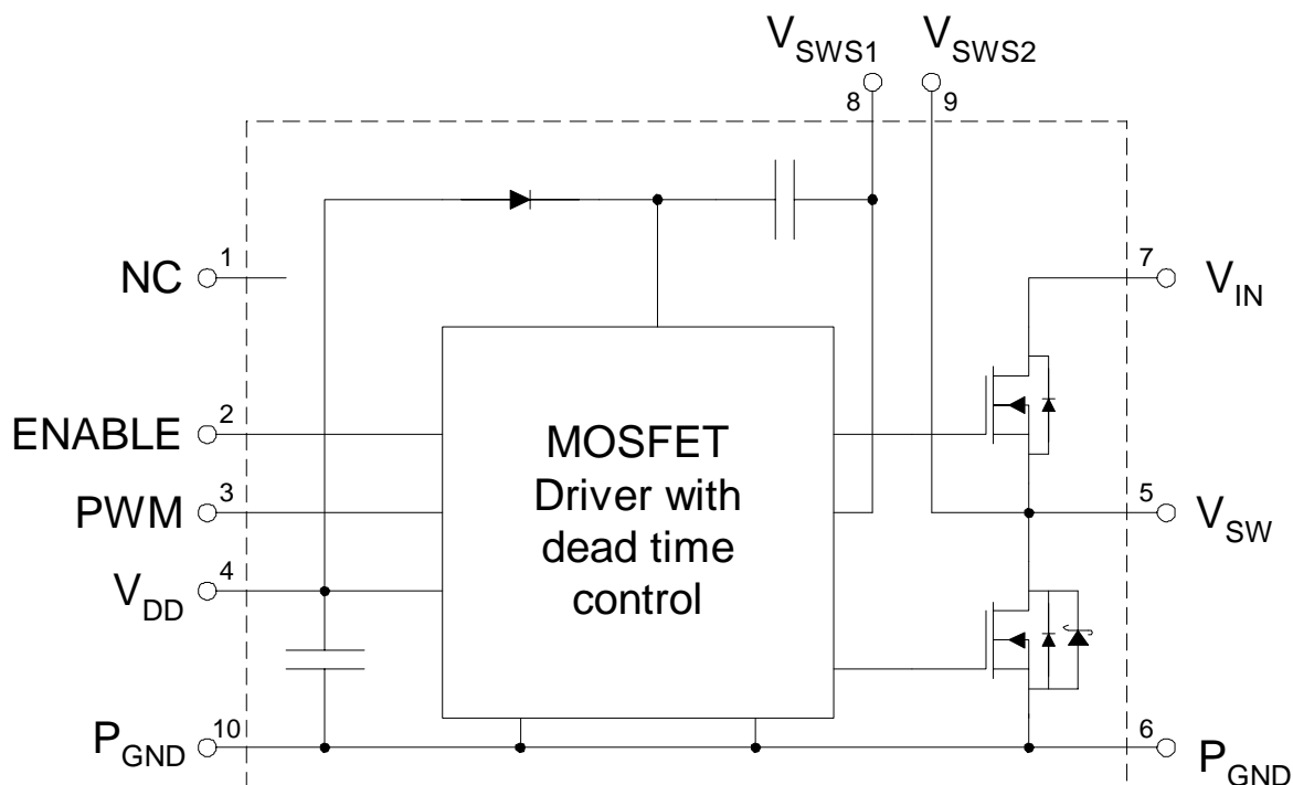
Figure 12 Internal Block Diagram
