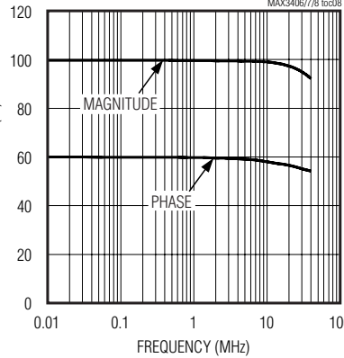
IMPEDANCE vs. FREQUENCY 100Ω MODE—MAX3406/MAX3408
