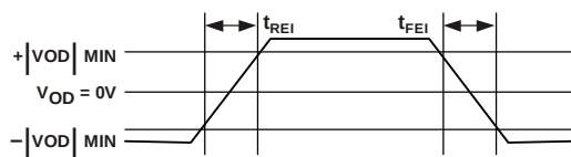
Figure 20. Link Ports—Differential Input Signals Transition Time
