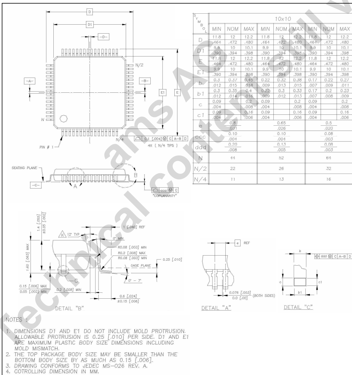
Figure 24 LQFP 10x10mm 0.5mm pitch
