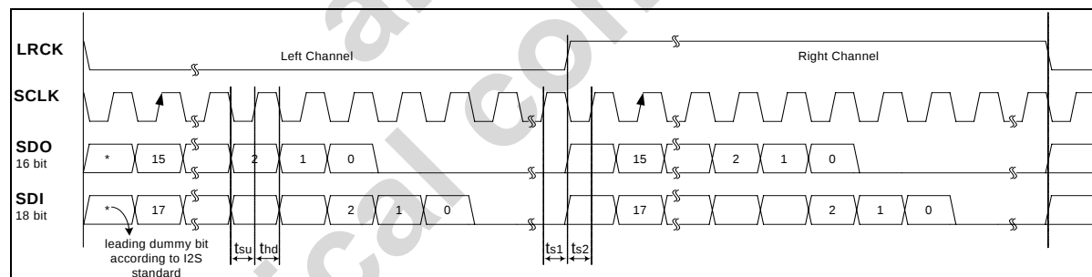
Figure 8 I2S_Timing
