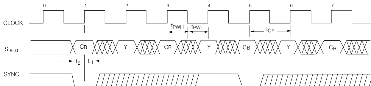
Fig. 9 Operation of SYNC Control Signal
