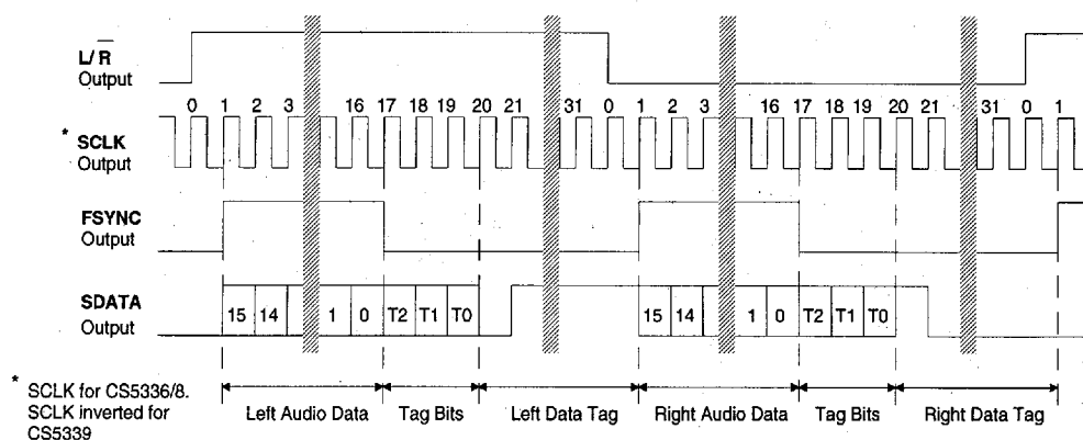
Figure 3. Data Output Timing - MASTER mode
