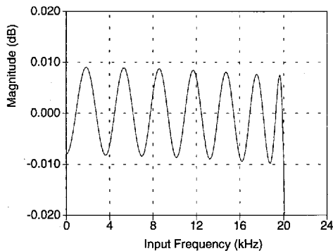
Figure 15. CS5336 Digital Filter Passband Ripple
