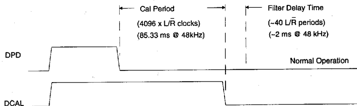
Figure 6. Initial Calibration Cycle Timing
