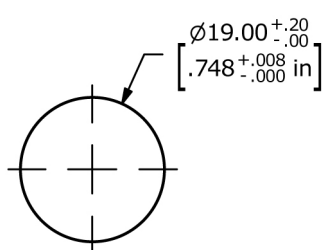
PANEL CUTOUT
