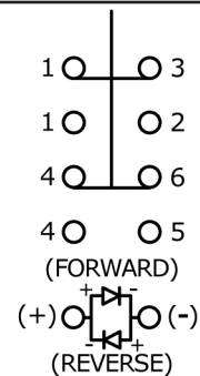
DPDT LED SCHEMATIC
