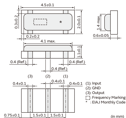
CSTNR_GH5C 4.00-7.99MHz
