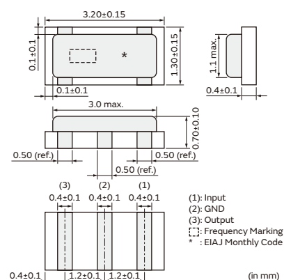
CSTNE_GH5C 8.00-13.99MHz
