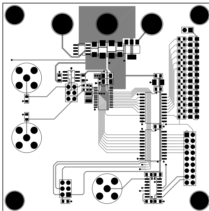
Figure 14c. Suggested Evaluation Circuit Board— Component Side Layout
