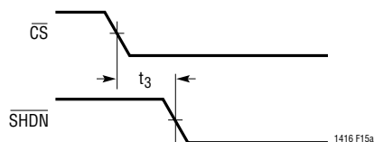
Figure 15a. \overline{CS} to \overline{SHDN} Timing
