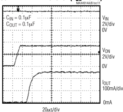
CURRENT-LIMIT RESPONSE ( V_{ON} RISING)
