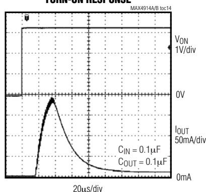
TURN-ON RESPONSE
