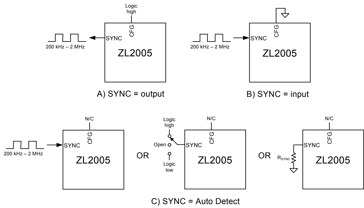
Figure 12. SYNC Pin Configurations
