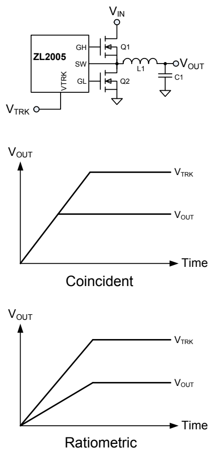
Figure 17. Tracking Modes
