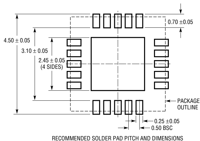
UF Package 20-Lead Plastic QFN (4mm × 4mm) (Reference LTC DWG # 05-08-1710)
