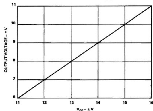
Output Voltage vs. V_{\text{CC}}
