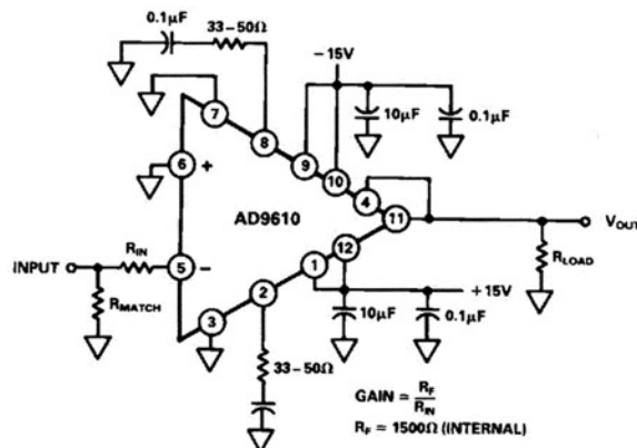
Figure 6. AD9610 Inverting Operation
