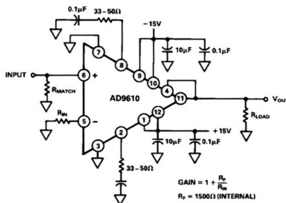
Figure 7. AD9610 Noninverting Operation
