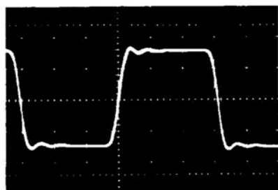
AD9610 Large-Signal Pulse Response
