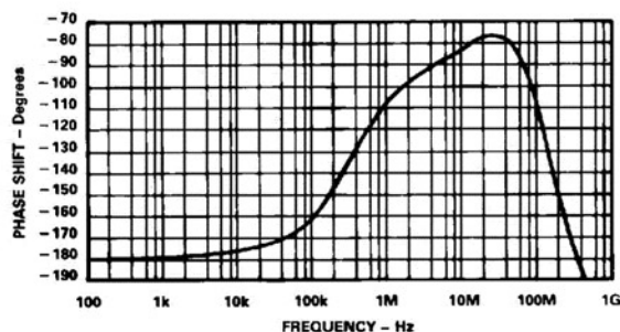
Small-Signal Output Phase Shift vs. Frequency ( G = -10 )
