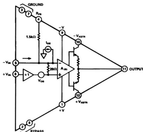
Figure 4. AD9610 Functional Circuit
