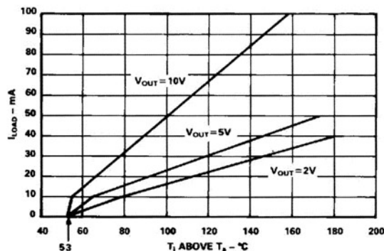
Figure 8. Junction Temp. Rise vs. Load Current
