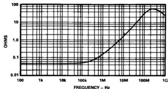
Small-Signal Output Resistance vs. Frequency ( G = -10 )
