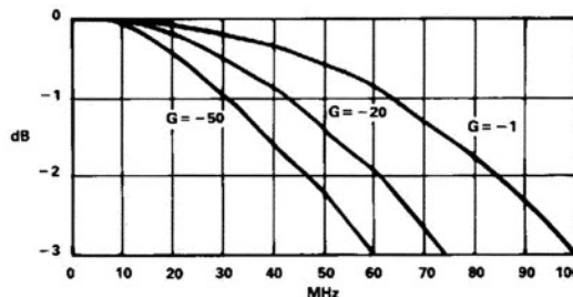
AD9610 Inverting Gain
