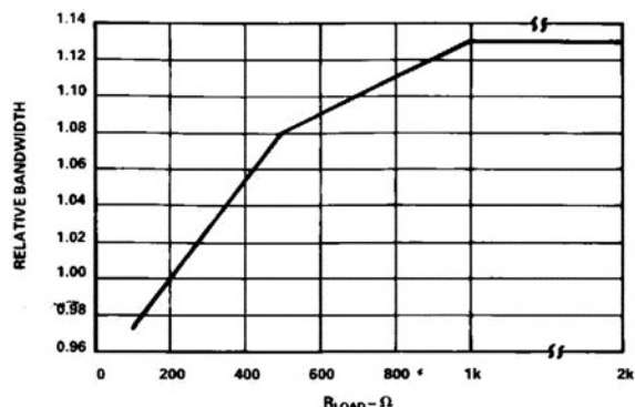
Bandwidth vs. Load
