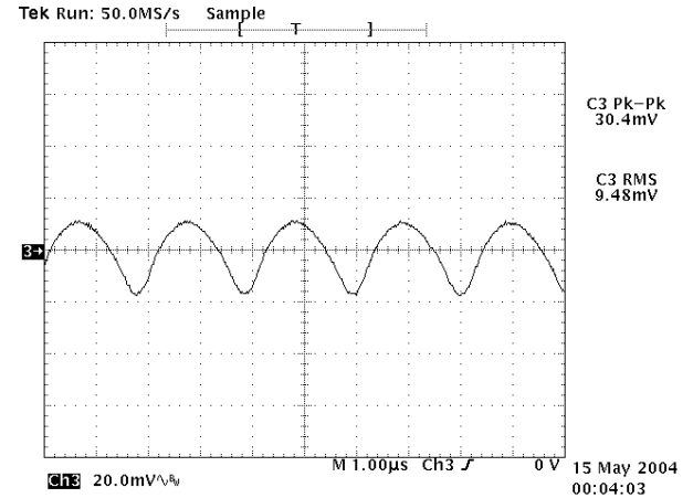
Figure 10: Output ripple & noise at 12Vin, 2.5V/8A out
