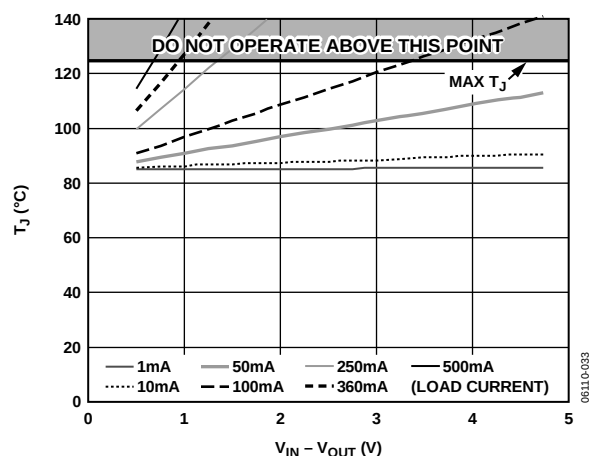
Figure 45. 0 mm² of PCB Copper, T_A = 85^\circ\text{C}
