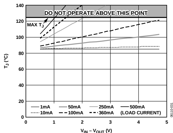
Figure 43. 300 mm² of PCB Copper, T_A = 85^\circ\text{C}
