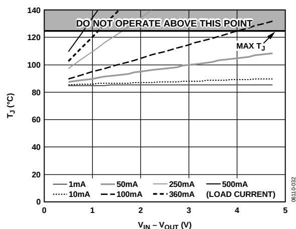
Figure 44. 100 mm² of PCB Copper, T_A = 85^\circ\text{C}
