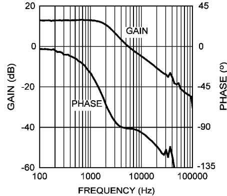
Figure 7-3. Modulator Gain and Phase
