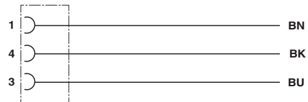
Contact assignment of the M5 socket
