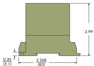
Dimensions for All CR6600 Series (shown)
