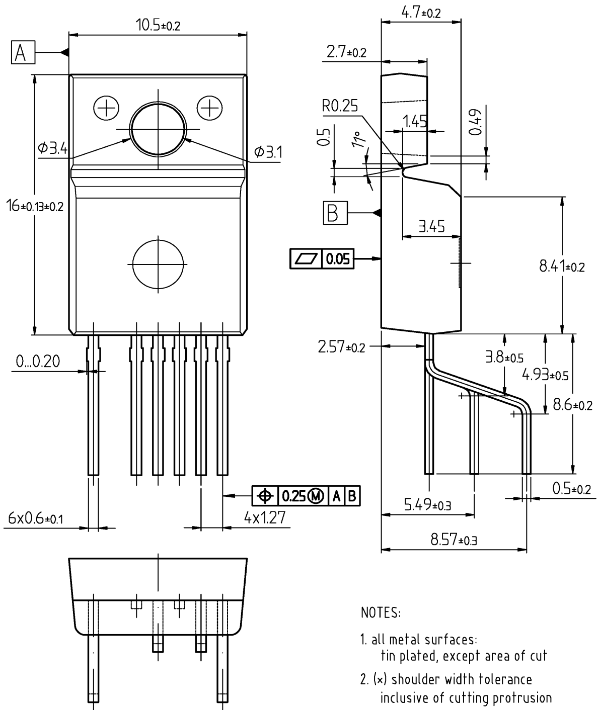
Figure 70 PG-TO220-6-347 (PB-free Plating Fullpak Package)
