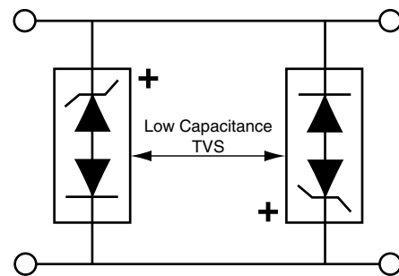
Application Note: Device must be used with two units in parallel, opposite in polarity as shown in circuit for AC signal line protection.
