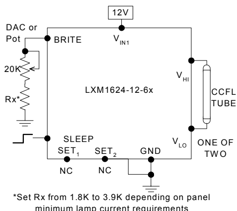
Figure 1 – Brightness Control (Output current set to maximum)
