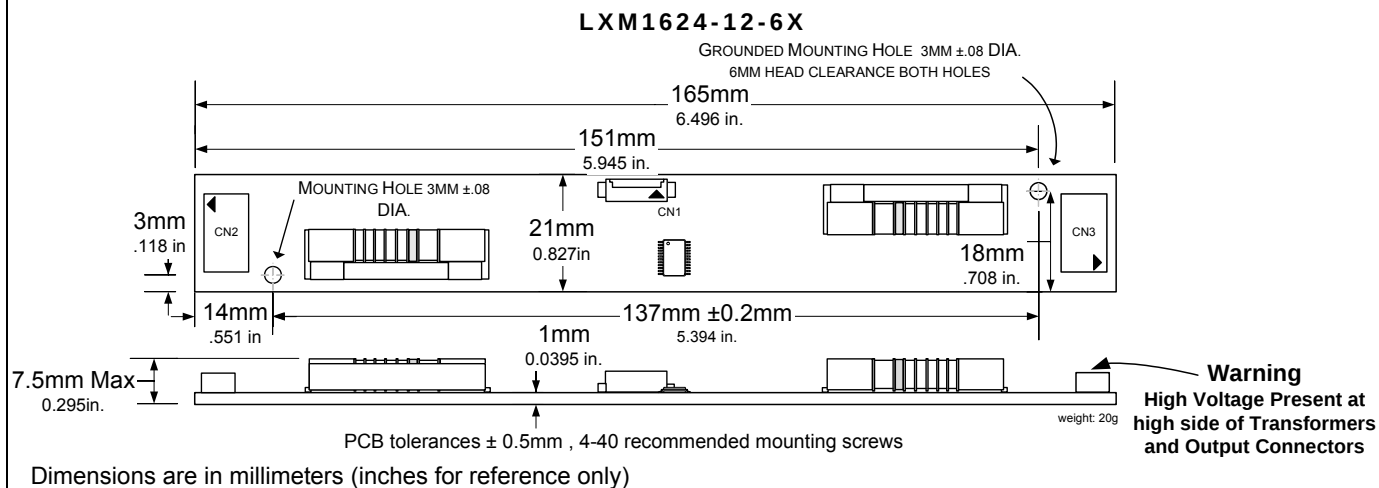
PHYSICAL DIMENSIONS
